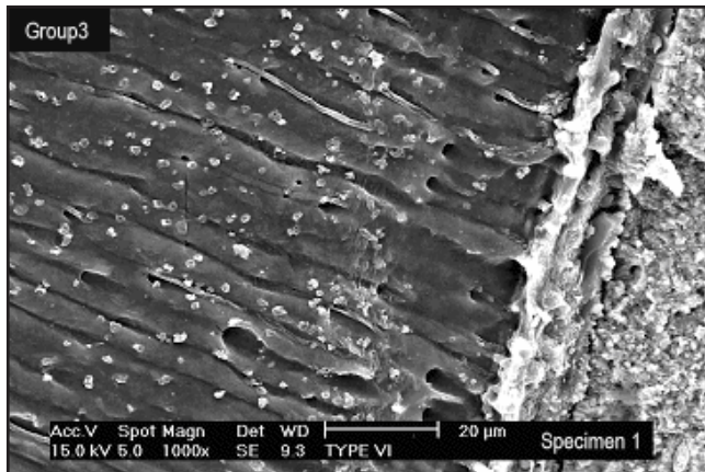
Fig 5: SEM Photograph showing hybrid layer in group 3 (specimen 1)
